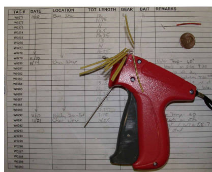
Figure 3. Dennison tag gun with tag strip inserted. Tags come in strips of 50 and T-bar anchor tags (top) measure 1.75 inches. Also shown is a waterproof data sheet for recoding catch information.
