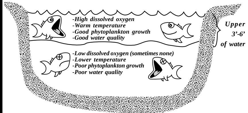
Figure 3 - Stratification (layering) of a fish pond in the summer.
