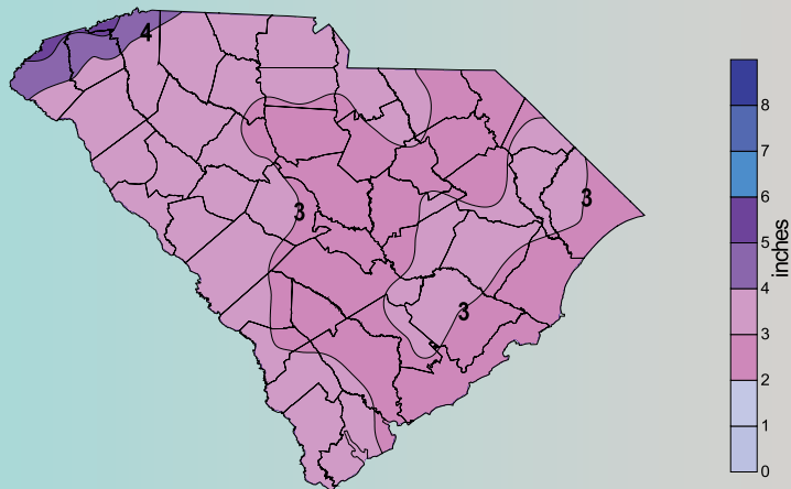
April Average Precipitation (1971-2000)
