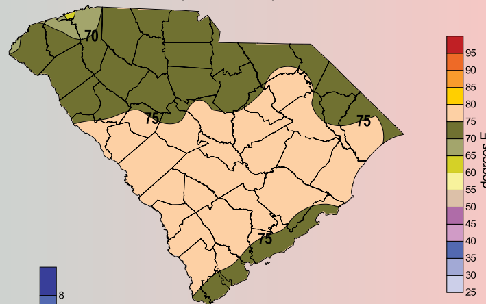
April Average Maximum Temperature (1971-2000)
