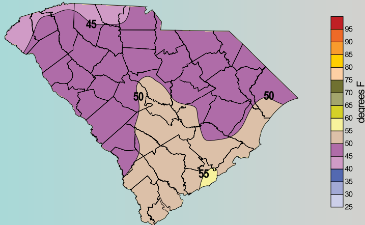
April Average Minimum Temperature (1971-2000)
