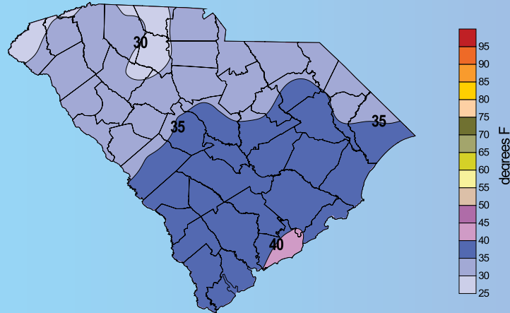
February Average Minimum Temperature (1971-2000)
