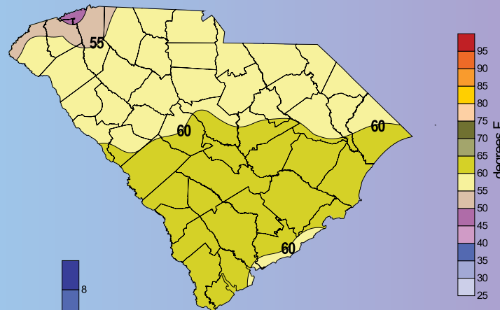
February Average Maximum Temperature (1971-2000)
