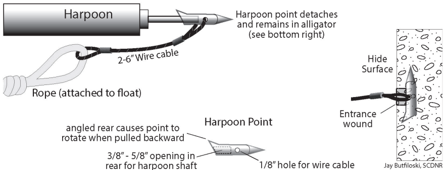
Diagram of a Commonly Used Harpoon Point
